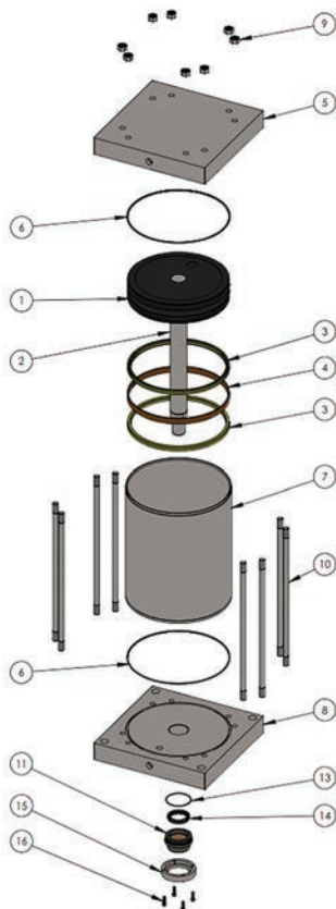
Figure 2 - RPSR Actuator Cylinder Exploded View
