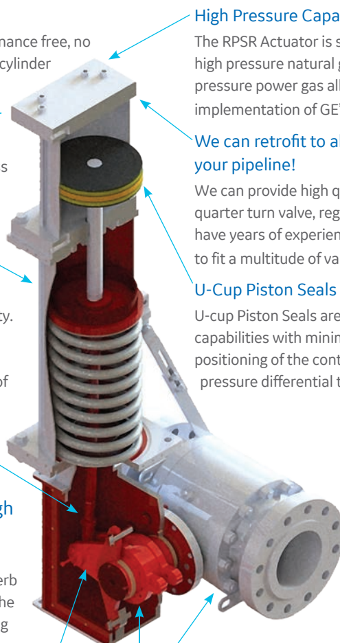
Figure 4 - Cutaway view of RPSR Actuator and Cylinder.
