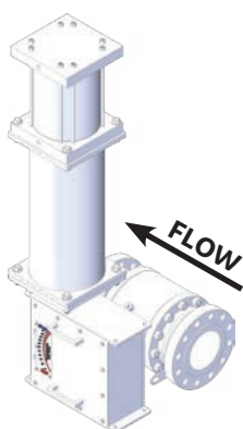
Mount #1 - Left Hand (Standard) with clean sweep feature
