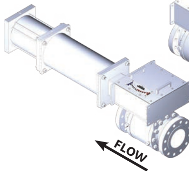
Mount #3 - Vertical Stem (Actuator Downstream)
