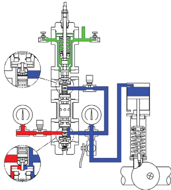
Figure 4.1 - Setpoint satisfied
