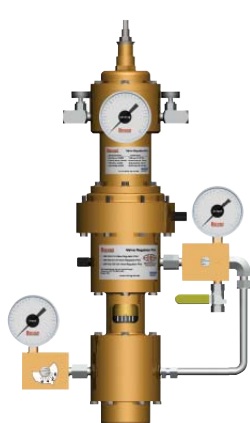
Figure 6.1 - VRP-175-SB-CH (Reverse-Acting)
