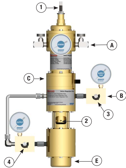
Figure 3 - Model VRP-600-SB-CH pressure control system. The VRP-SB-CH is specifically designed for use in natural gas pressure regulation and provides a simple, economical alternative to the controller and positioner combination.
